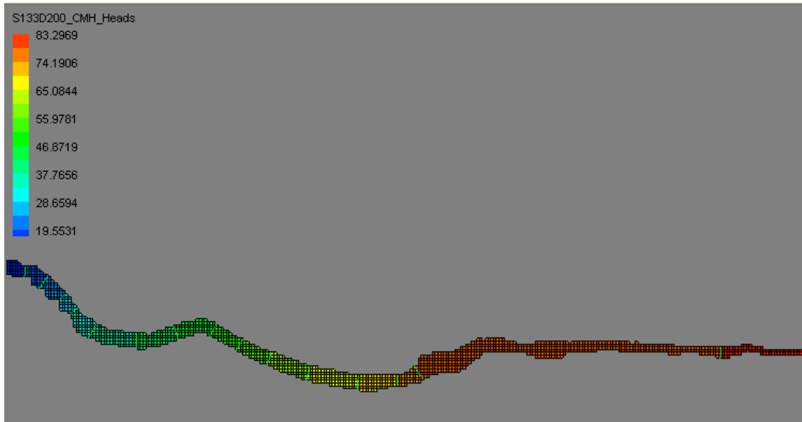
Figure 3.5 MODFLOW output
