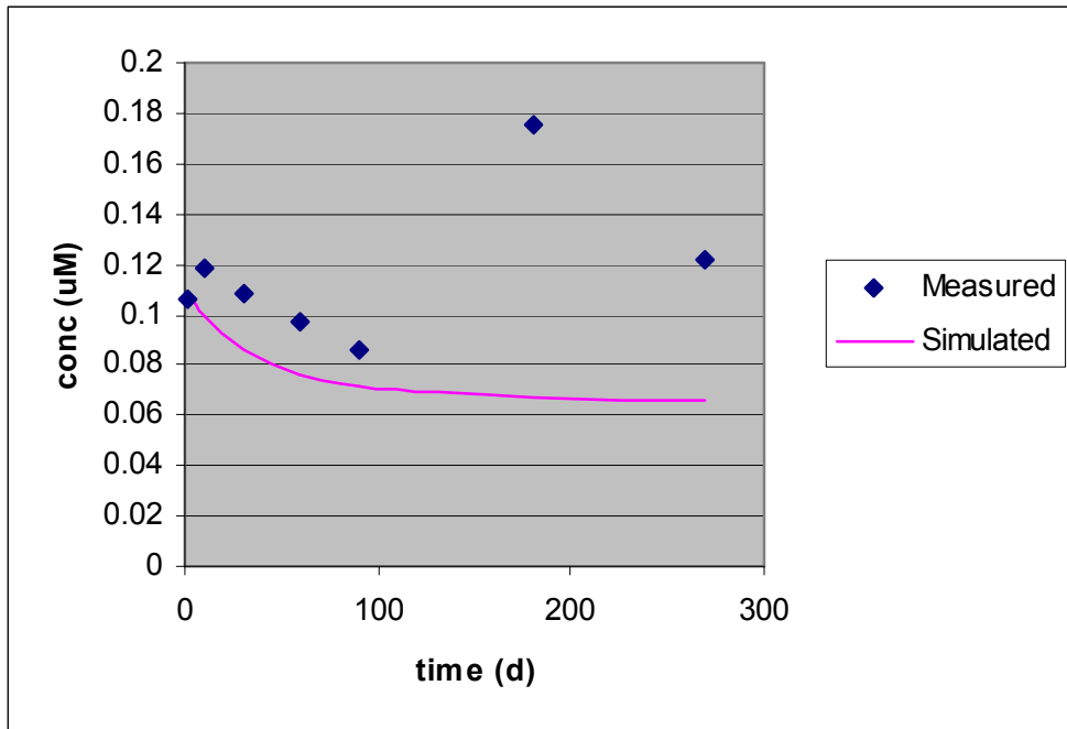
Figure 4.28 Measured and simulated VC values at 14-MW-3
