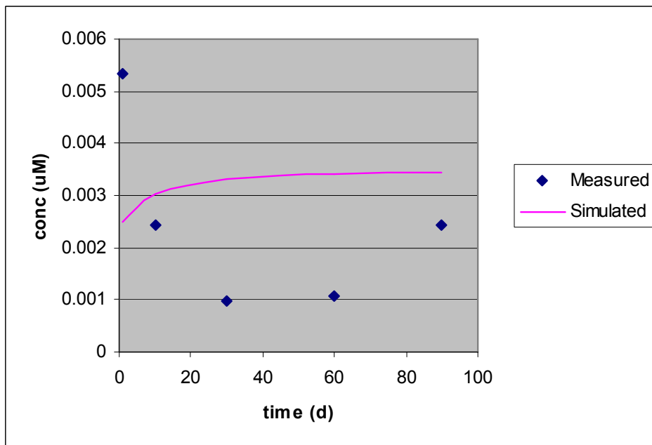
Figure 4.15 Measured and simulated TCE values at 14-MW-10
