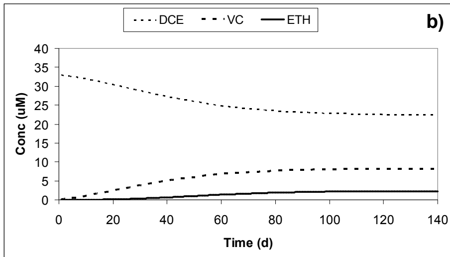
Figure 4.12 Modeled and simulated reductive dehalogenation of DCE from (a) Lee et al. (2004) compared with (b) batch simulations of the dual-Monod kinetic submodel developed for this study
