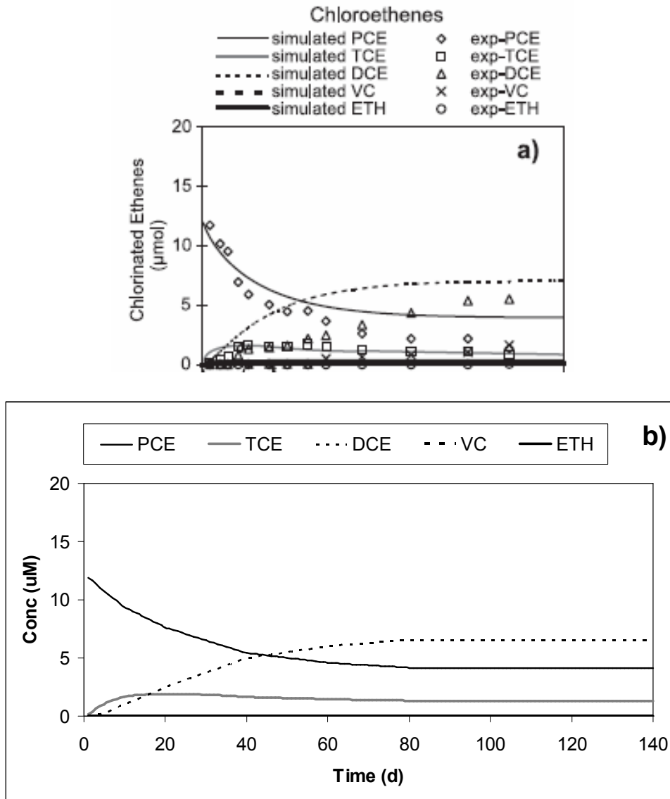
Figure 4.11 Modeled and simulated reductive dehalogenation of PCE from (a) Lee et al. (2004) compared with (b) batch simulations of the dual-Monod kinetic submodel developed for this study
